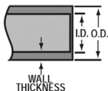
SCHEDULE 80 PIPE DIMENSIONS ASTM D 1785
