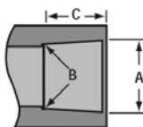
SCHEDULE 80 SOCKET DIMENSIONS ASTM D 2467
