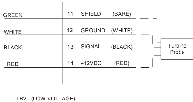
Figure 18 Autotrol Turbine Meter
