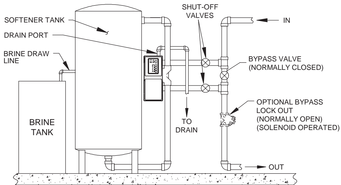
Figure 20 Normal Installation
