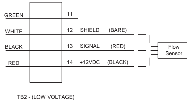
Figure 19 Signet Flow Sensor
